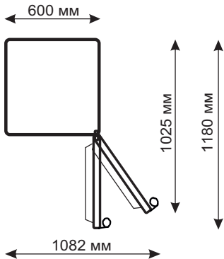
Dimensions of the cooling unit
