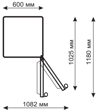
Dimensions of the cooling unit
